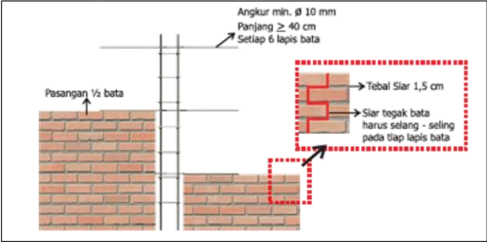
Gambar 40. Detail Dinding
